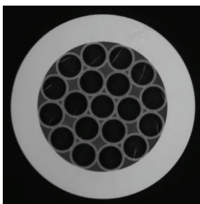
19-to-1 Combiner
